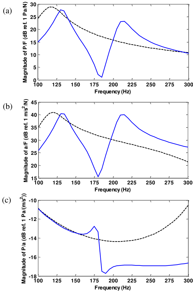
Figure 5: Magnitude of FRFs obtained from the simulation results, the dashed curve represents the aluminum panel and the solid curve represents the SAM panel, (a) Magnitude of P/F ; (a) Magnitude of a/F ; (a) Magnitude of P/a .
